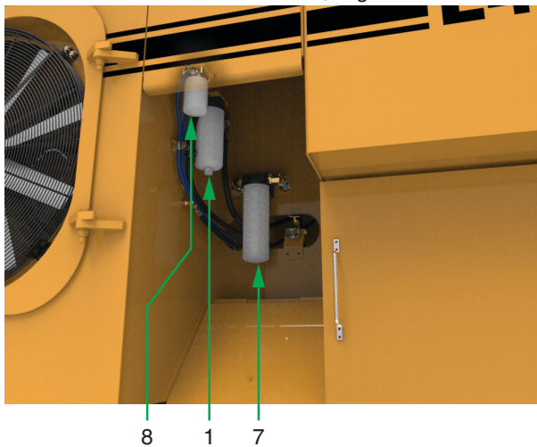
Filters Mounted Remotely. Access at Chassis, Right Side.
