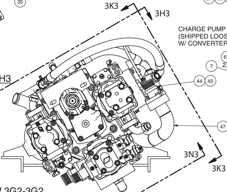
VIEW 3G2-3G2 PUMP INSTL DETAIL
