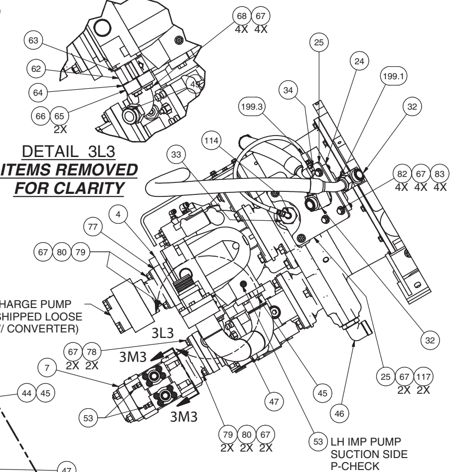
SECTION 3K3-3K3 RH IMP PUMP FITTING INSTL
