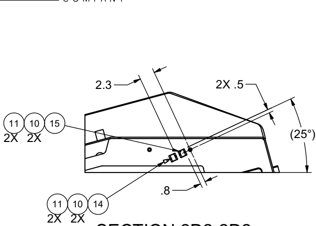
SECTION 2D2-2D2
