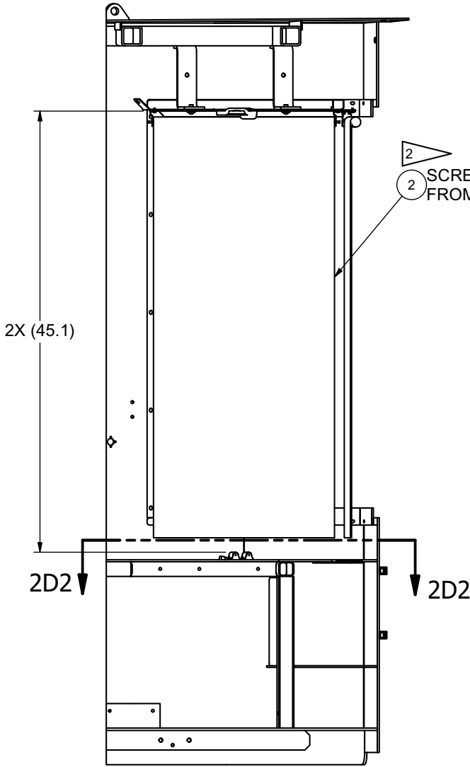
SECTION 2G1-2G1
