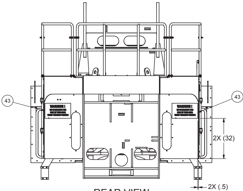
REAR VIEW
