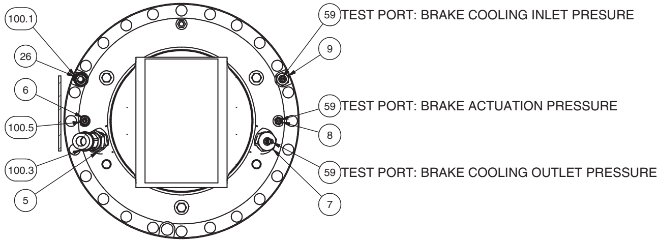
SECTION 3C1-3C1 LH BRAKE HUB PLUMBING SIMILAR SETUP FOR RH BRAKE HUB
