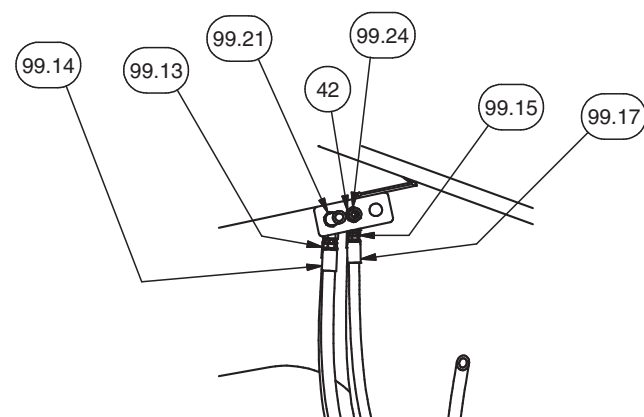
SECTION 2L1-2L1 BRAKE BULKHEAD PLATE
