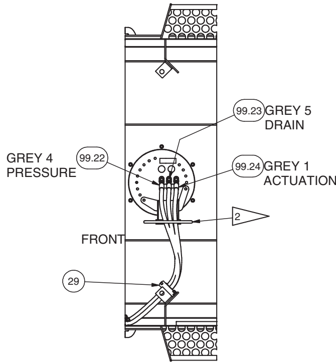
SECTION 3D1-3D1 SWIVEL PLATE
