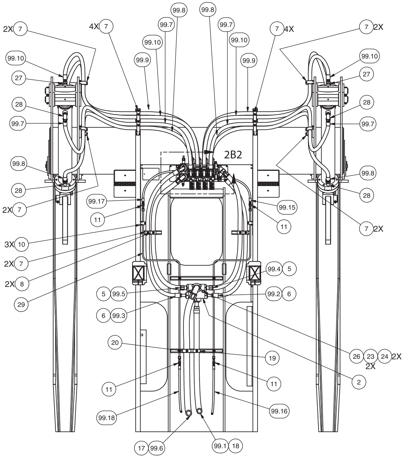
SECTION 2A1-2A1 SOME PARTS REMOVED FOR CLARITY
