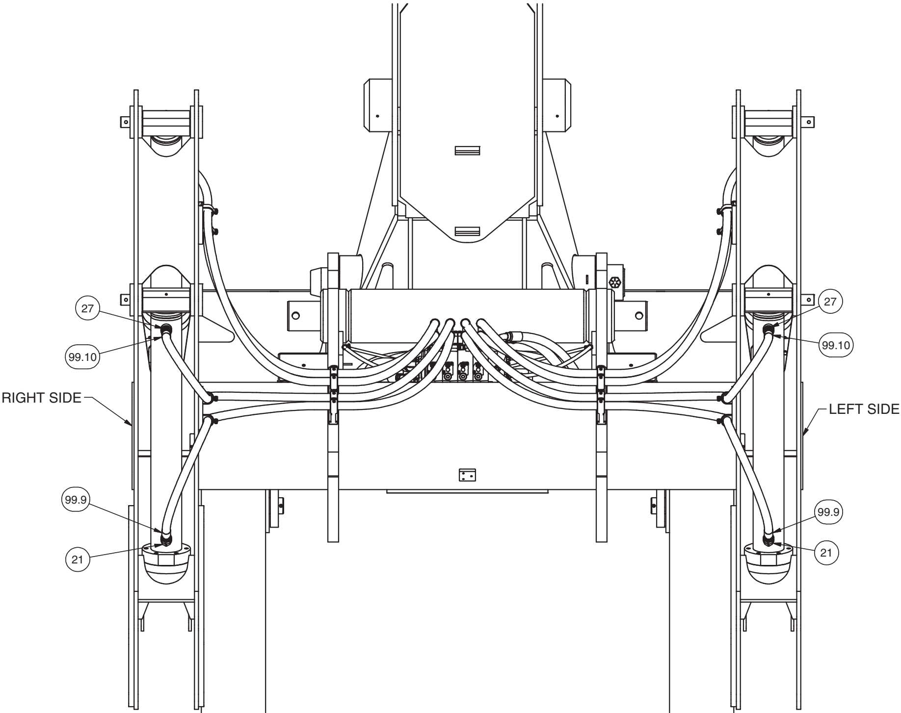
TOP VIEW
