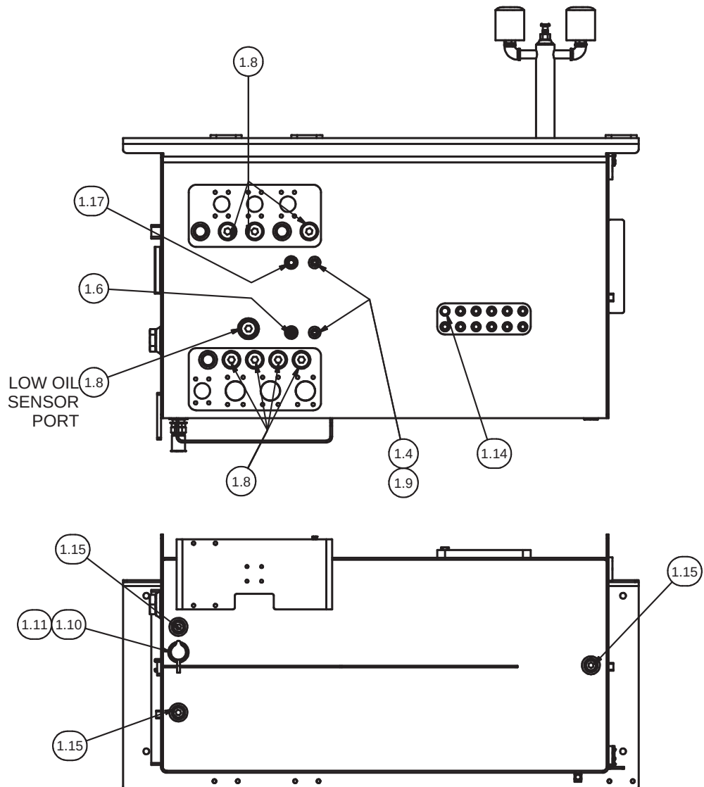
SECTION A-A RETURN FILTERS IN RETURN BOX
