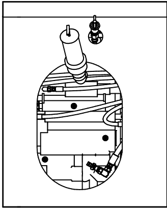
DETAIL A FILL AND DIPSTICK LOCATION
