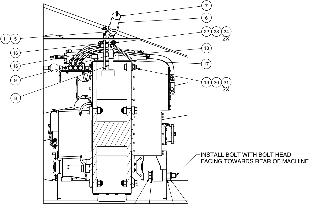
SECTION C-C 4X TRANSMISSION BOLTS
