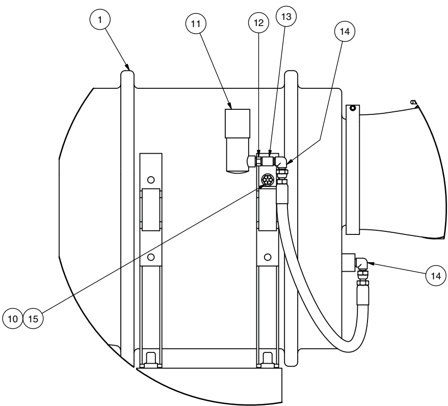
DETAIL 2C2
