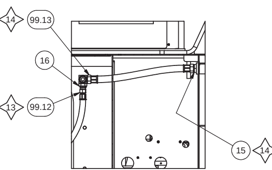
SECTION 2C1-2C1 HYD. COOLER RETURN TO TANK INSTL
