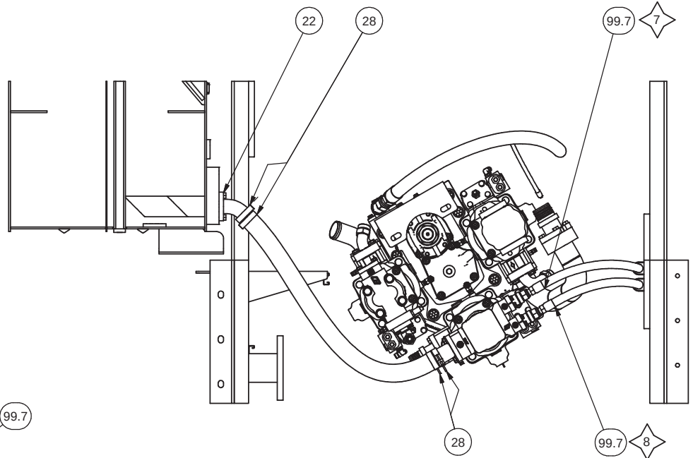
SECTION 2G1-2G1 FAN DRIVE PUMP PLUMBING INSTL
