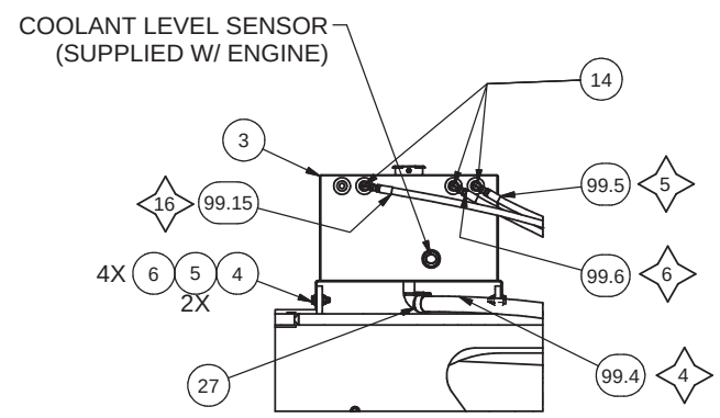
SECTION 2D1-2D1 SURGE TANK INSTL
