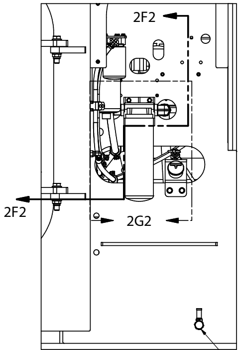
VIEW 2D1-2D1
