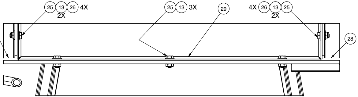
DETAIL 2B2
