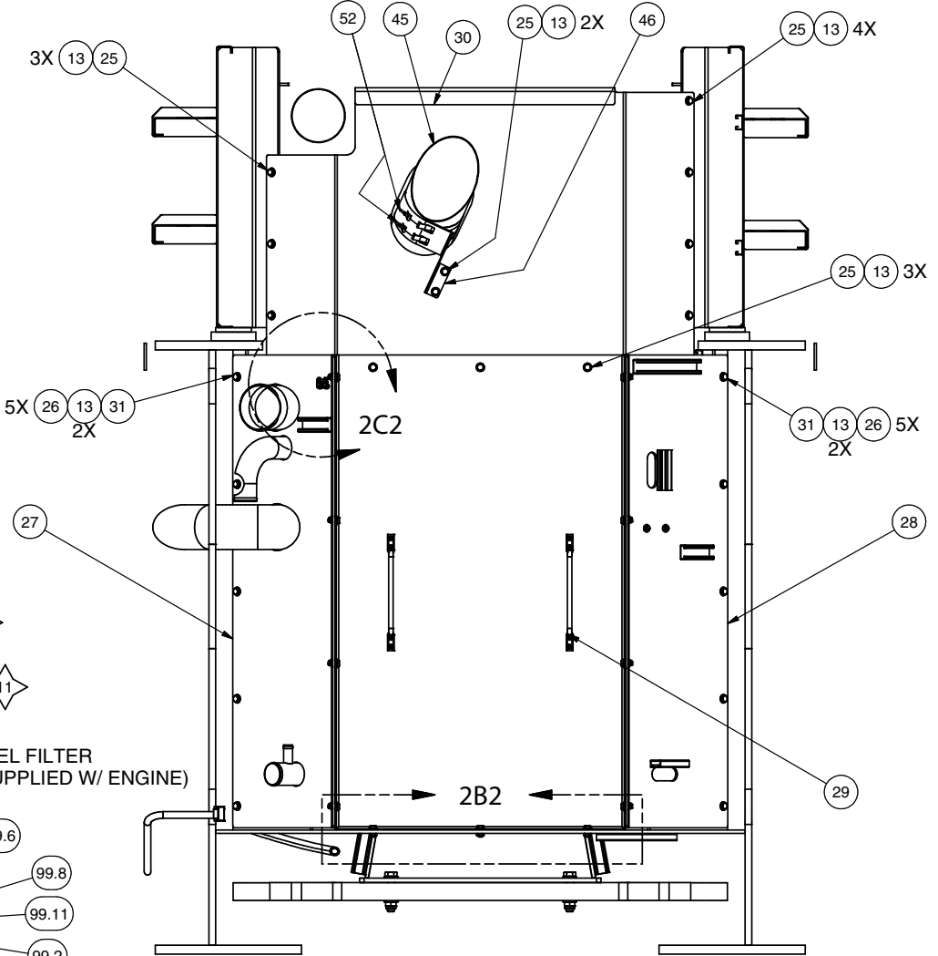
SECTION 2A1-2A1 BULKHEAD/ISOLATION PLATE INSTL VIEW ROTATED 90°
