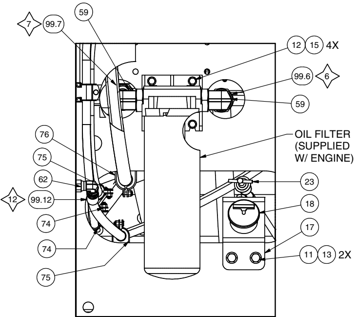
DETAIL 2G2 OIL FILTER INSTL
