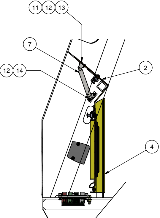
SECTION B-B VIEW ROTATED
