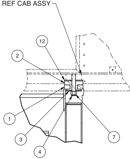
DETAIL B 4 PLACES
