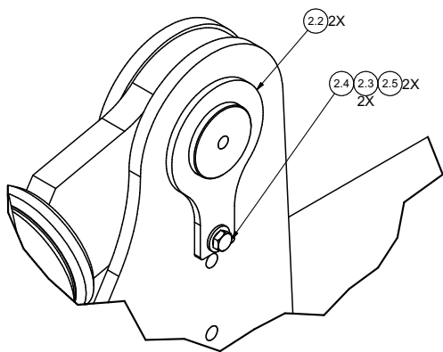
DETAIL A TILT CYL BASE RETENTION
