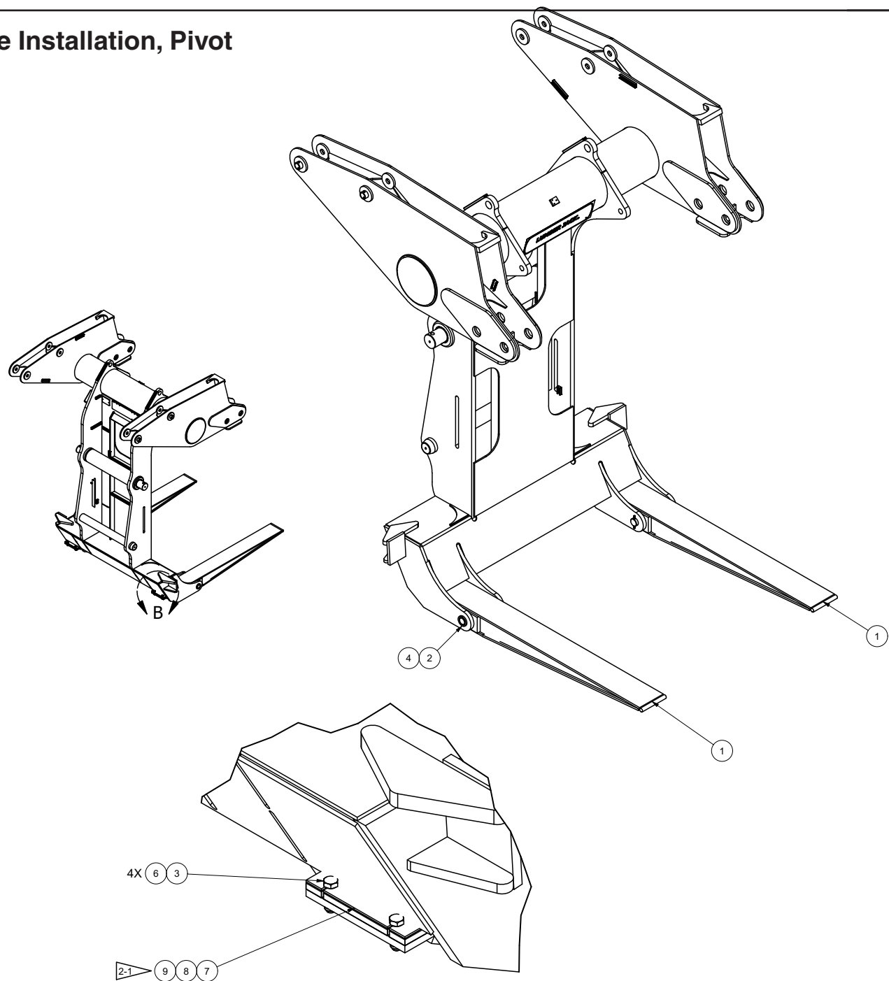
DETAIL B TINE SHIMS BOTH TINES
