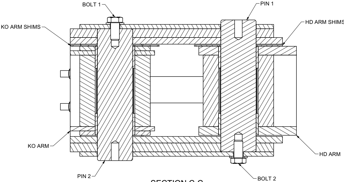
SECTION C-C ANTI-ROTATION PINS INSTALLATION VIEW CROPPED FOR CLARITY
