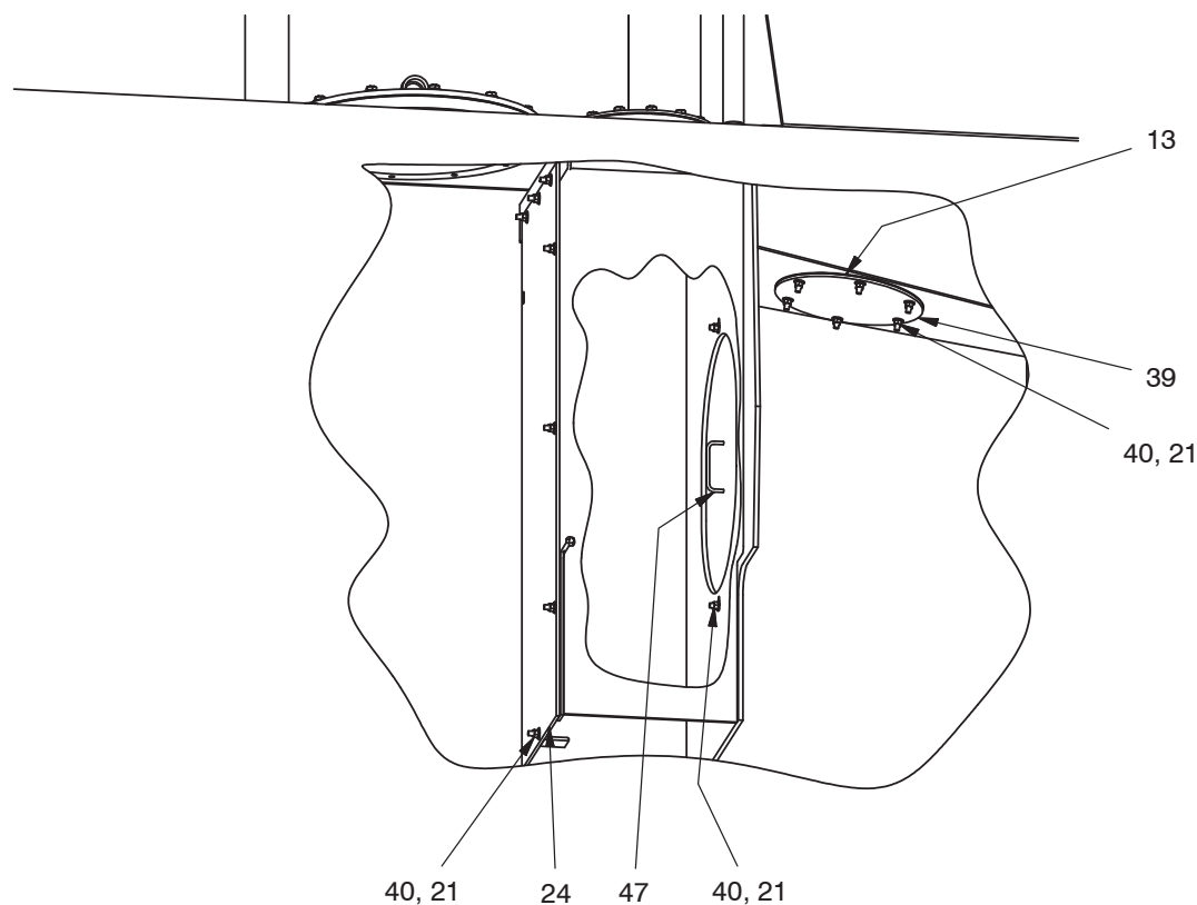
Detail Inside Hydraulic Tank
