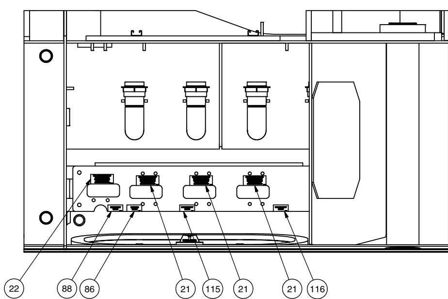
SECTION 3K4-3K4
