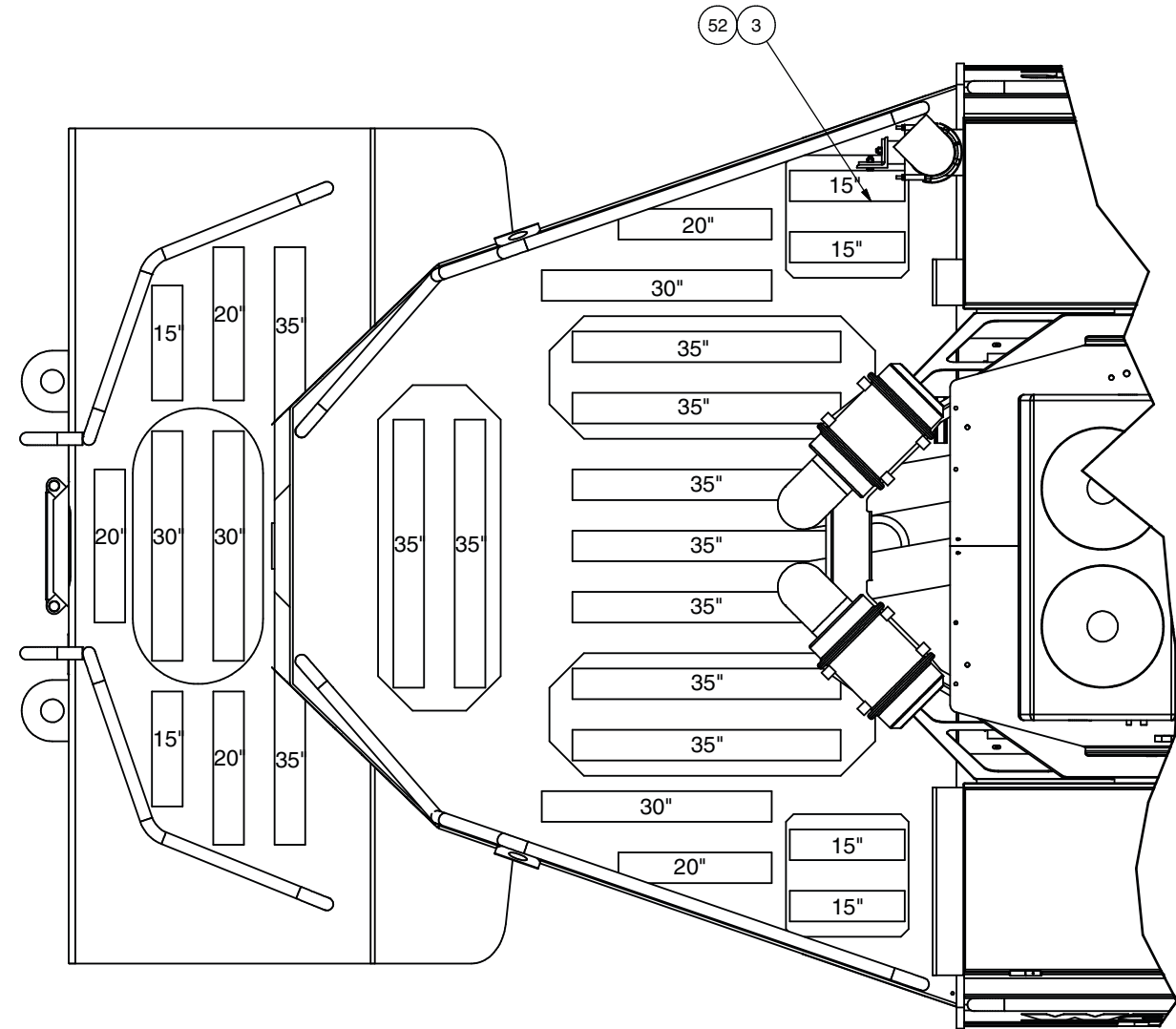
DETAIL 2F4
