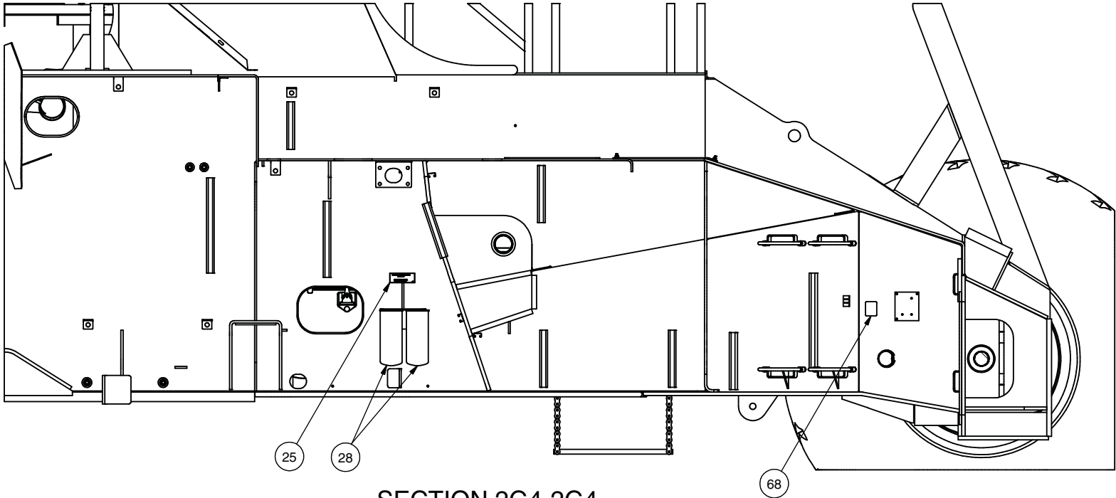
SECTION 2G4-2G4
