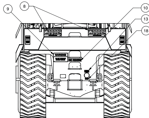
VIEW 2B2-2B2
