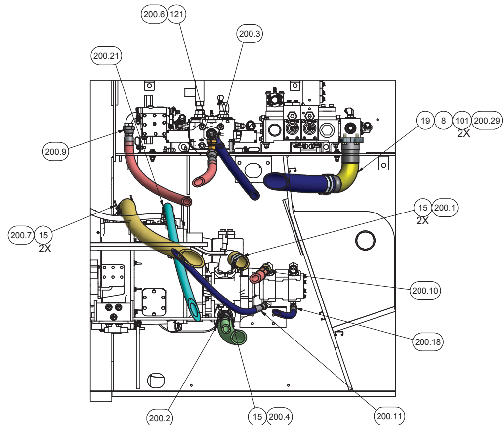
SECTION 2C1-2C1 PUMPS & VALVES
