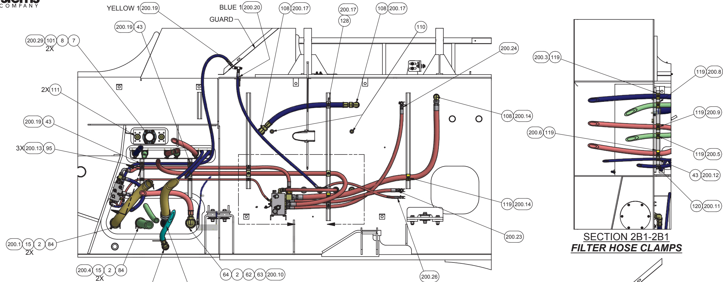
SECTION 2A1-2A1
