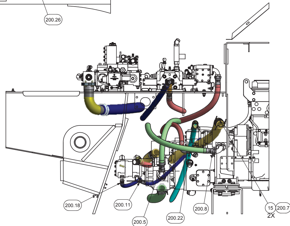
SECTION 2D1-2D1 PUMPS & VALVES
