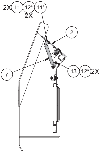
SECTION A-A VIEW ROTATED
