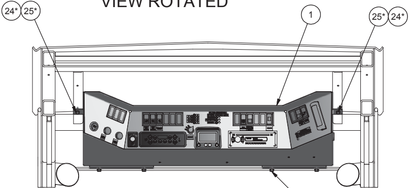
SECTION E-E OVERHEAD CONSOLE VIEW ROTATED
