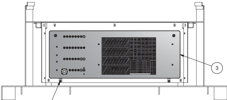
SECTION F-F ELECTRICAL PANEL
