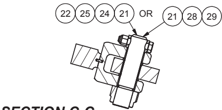
SECTION C-C 2 PLCS
