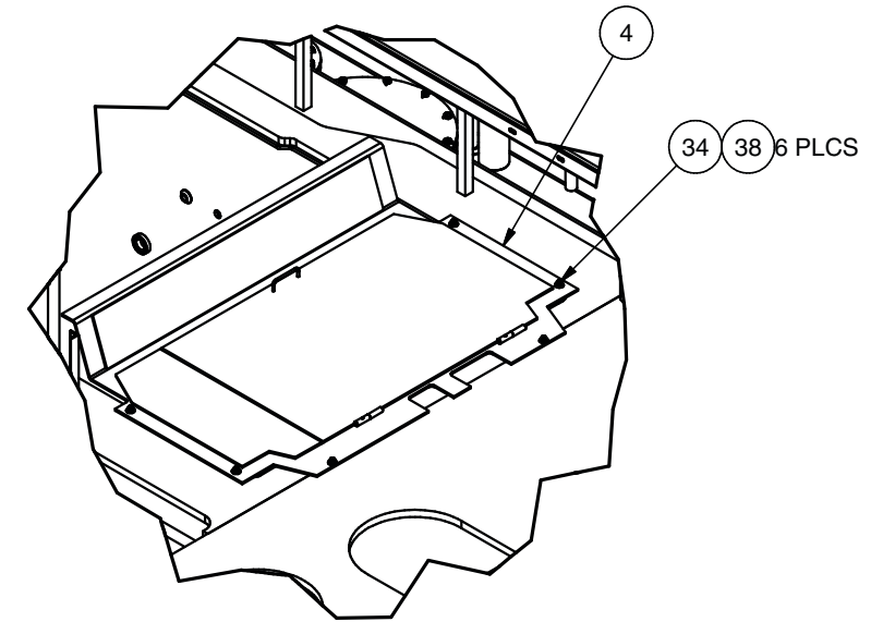
DETAIL 1C
