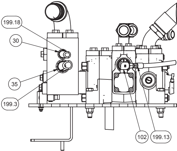
DETAIL 3E2 DUMP VALVE
