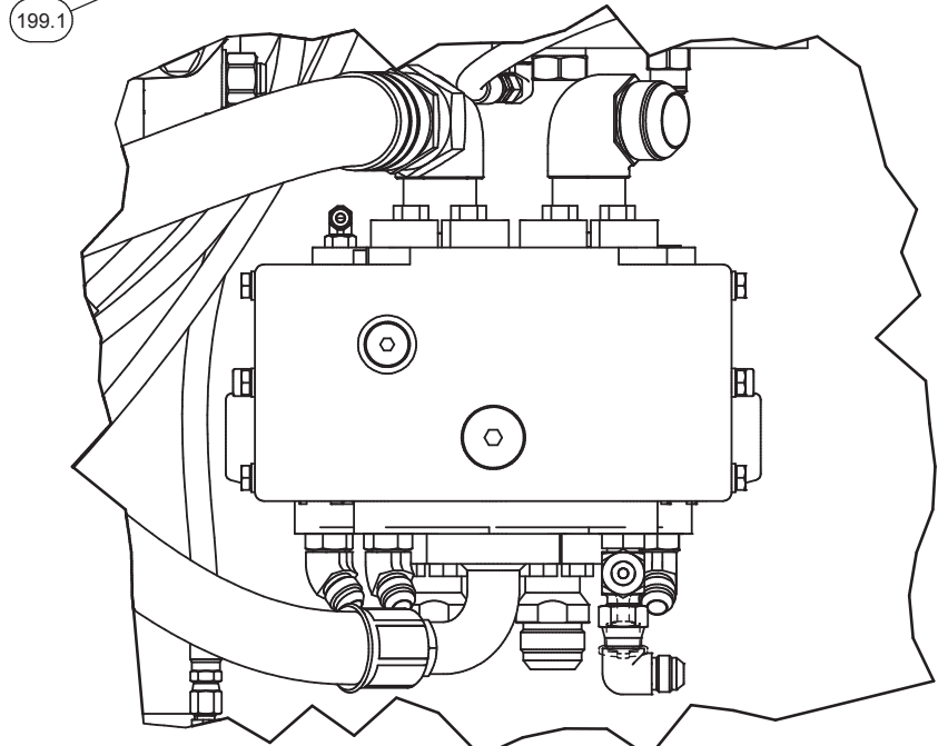
DETAIL 4G2
