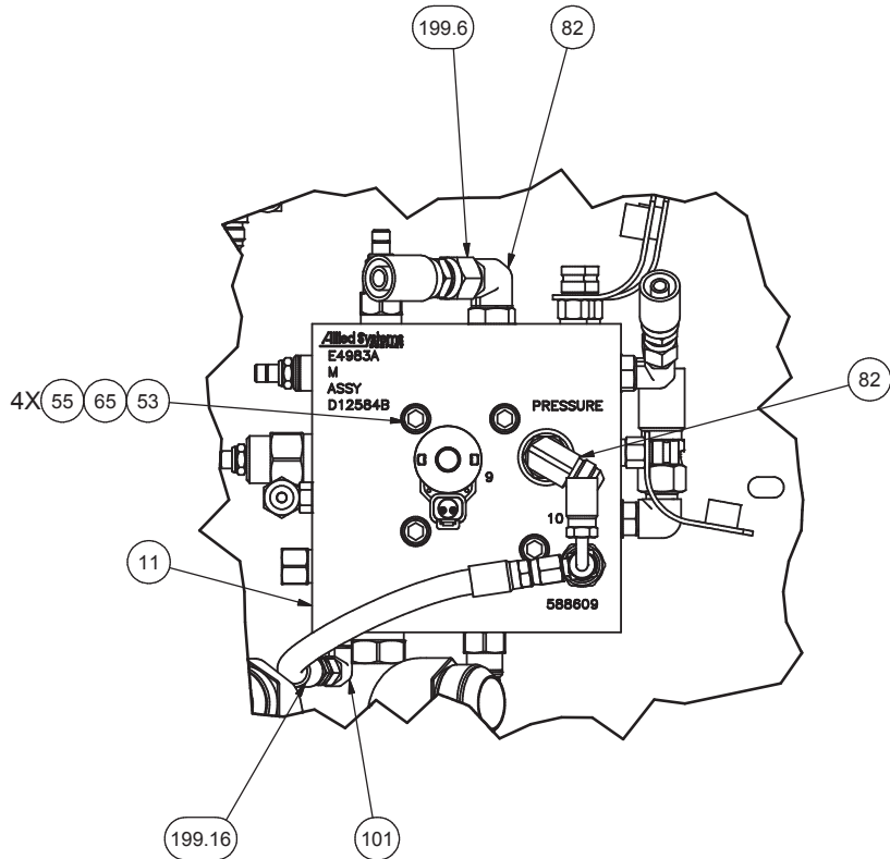
DETAIL 4H2 BRAKE ACCUMULATOR CHARGE MANIFOLD
