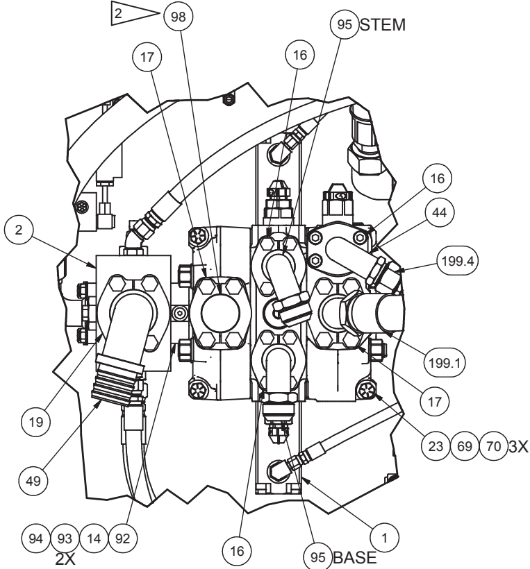
DETAIL 3E2 DUMP VALVE
