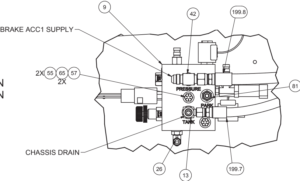
DETAIL 4J2 BRAKE MANIFOLD
