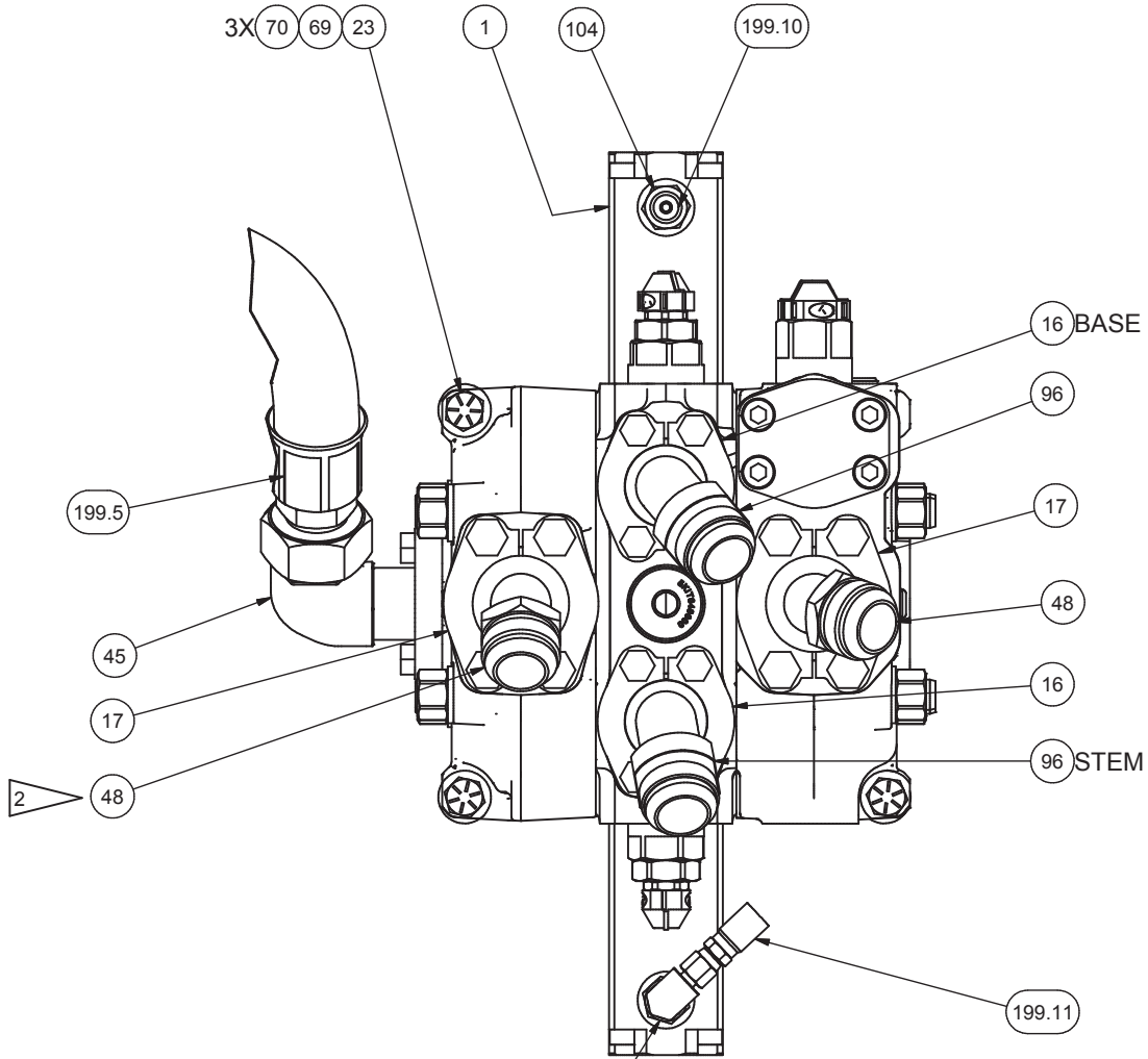
DETAIL 3F2 HOIST VALVE
