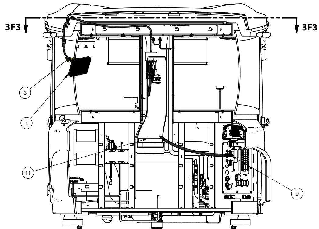
SECTION 3F3-3F3
