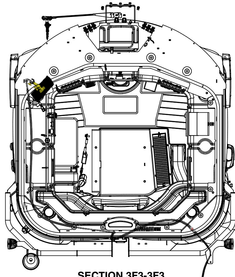
SECTION 3F3-3F3
