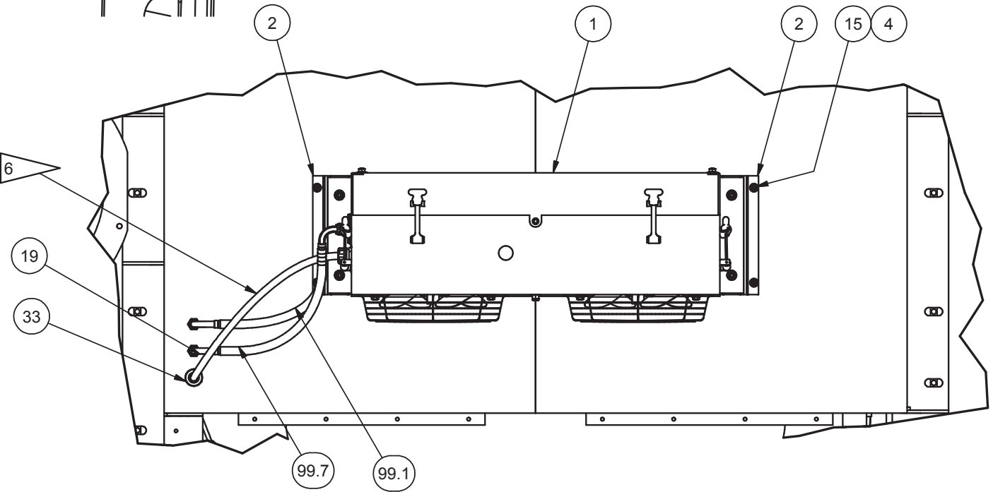
DETAIL 1B1
