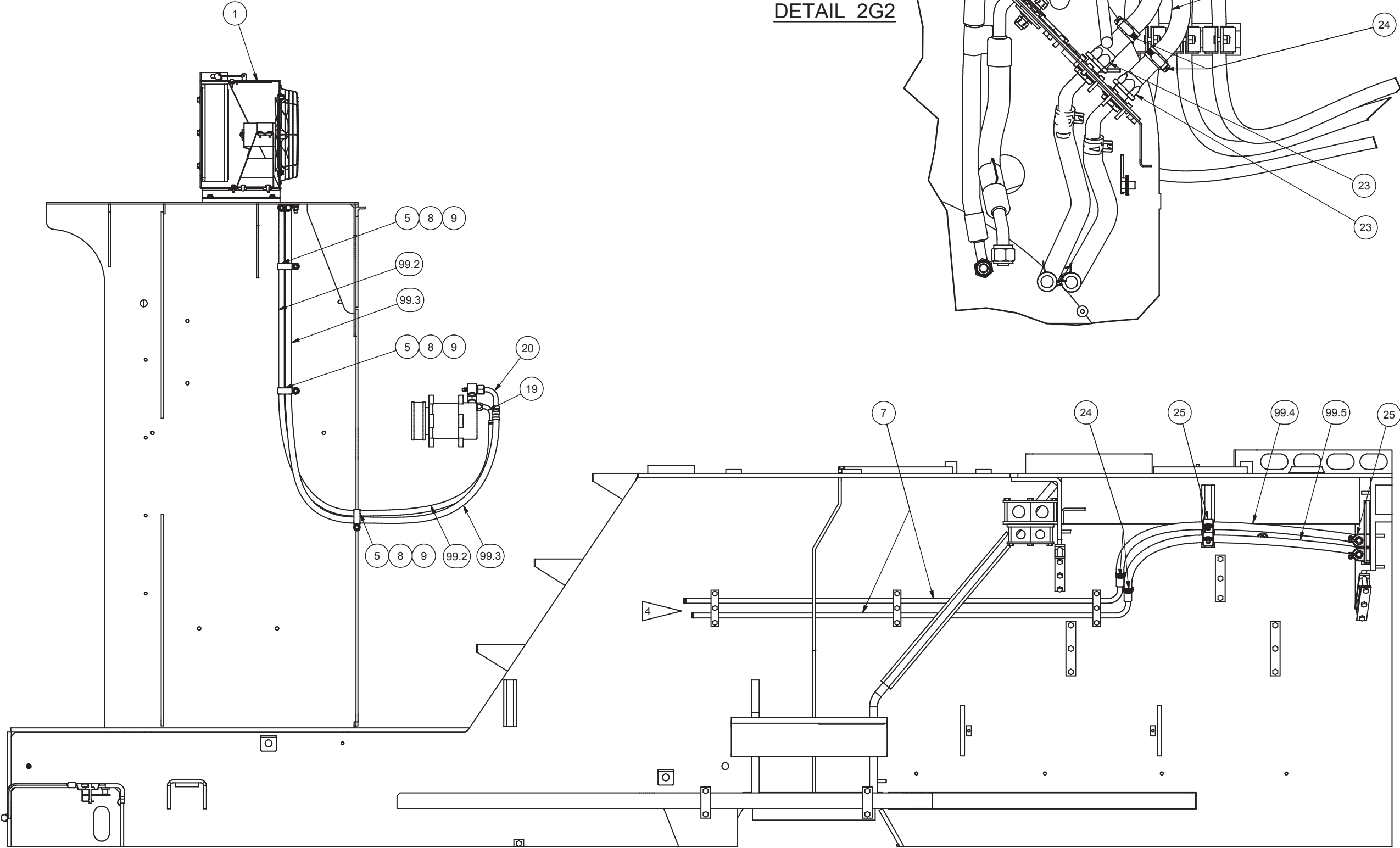
SECTION 2D1-2D1
