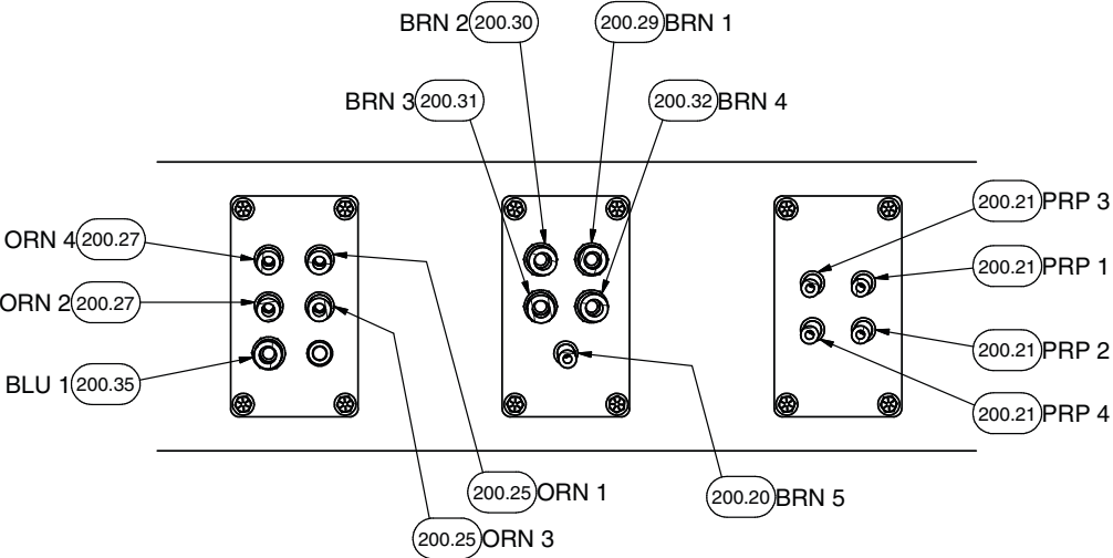
SECTION 3A3-3A3 BAFFLE BULKHEAD
