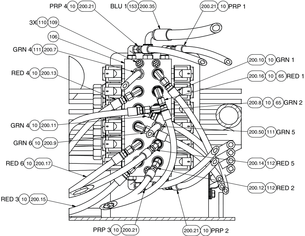
SECTION 3C3-3C3 IMPL FUNCTION MANIFOLD
