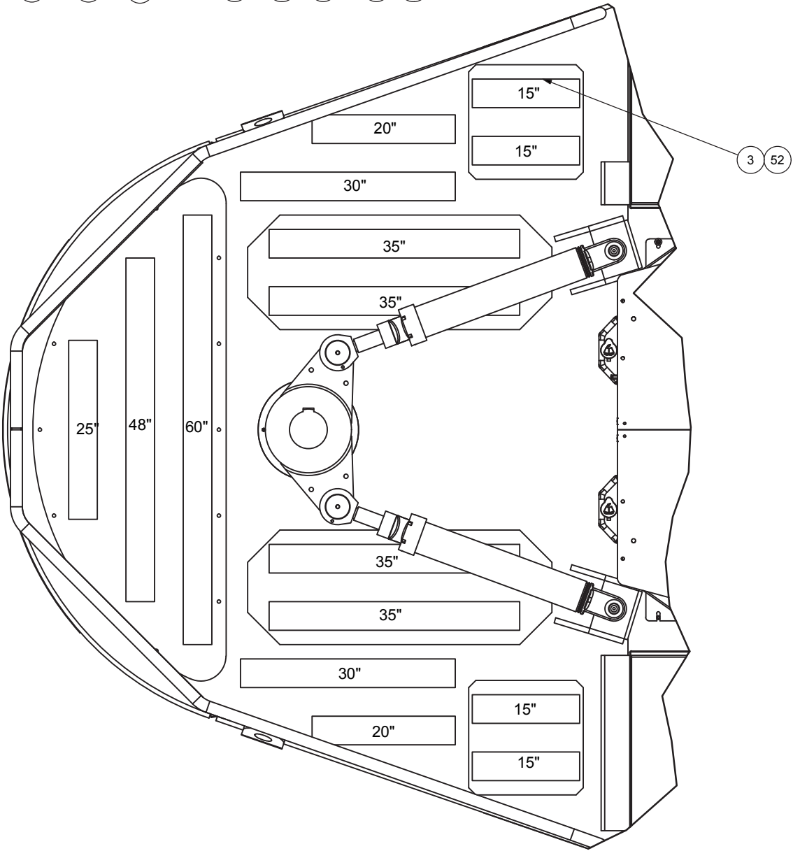
DETAIL 2F4
