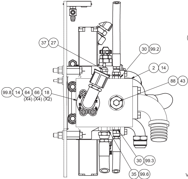
DETAIL 2D1 DUMP VALVE
