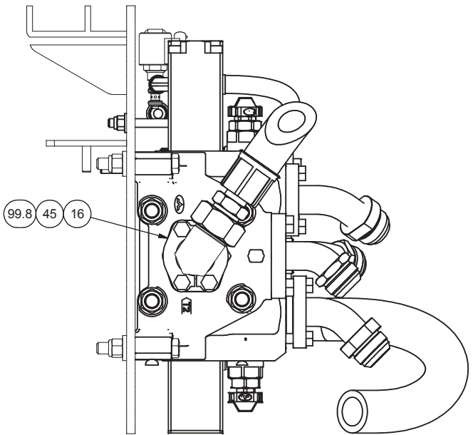
DETAIL 2E1 HOIST VALVE
