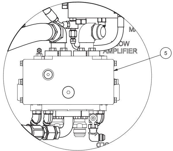
DETAIL 2C1 STEERING FLOW AMP
