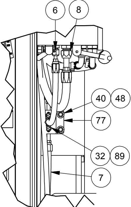
DETAIL 4G
