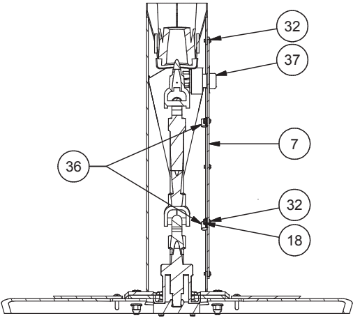
SECTION A1-A1
