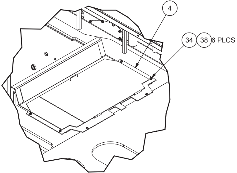
DETAIL 1C
