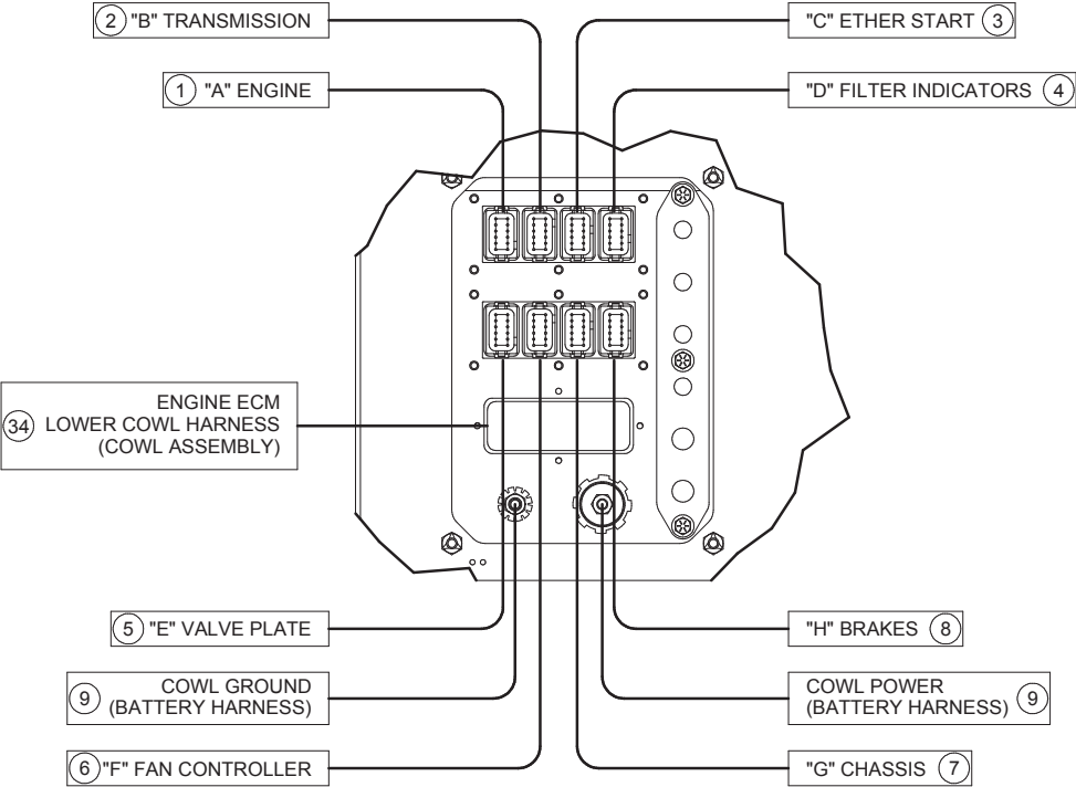
CAB HARNESS
