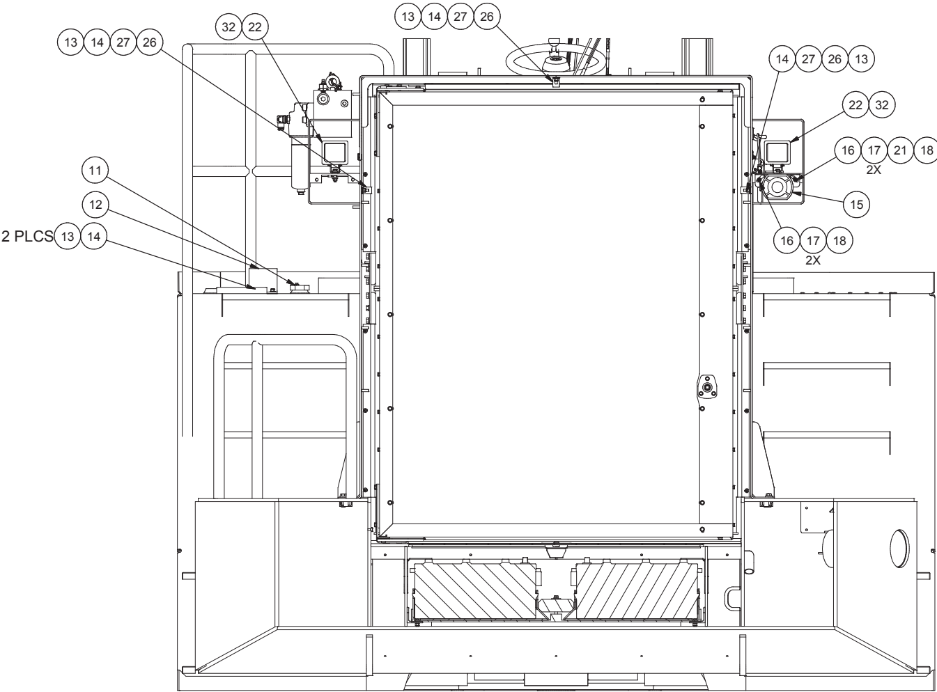
SECTION 2B-2B LIGHTS & BACK-UP ALARM
