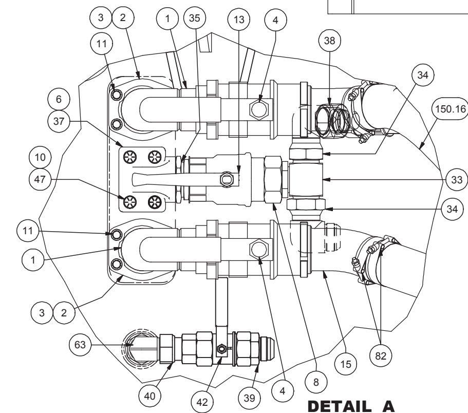
DETAIL A
