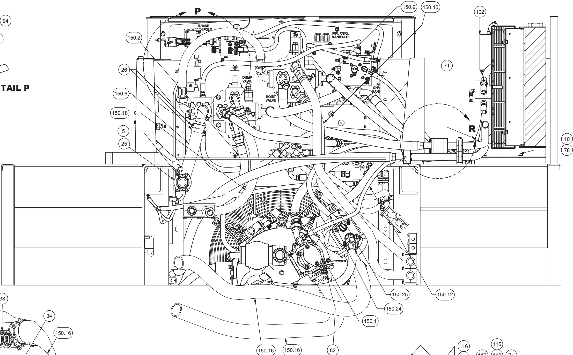
SECTION N-N
