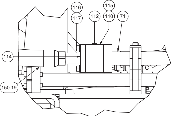
DETAIL R
