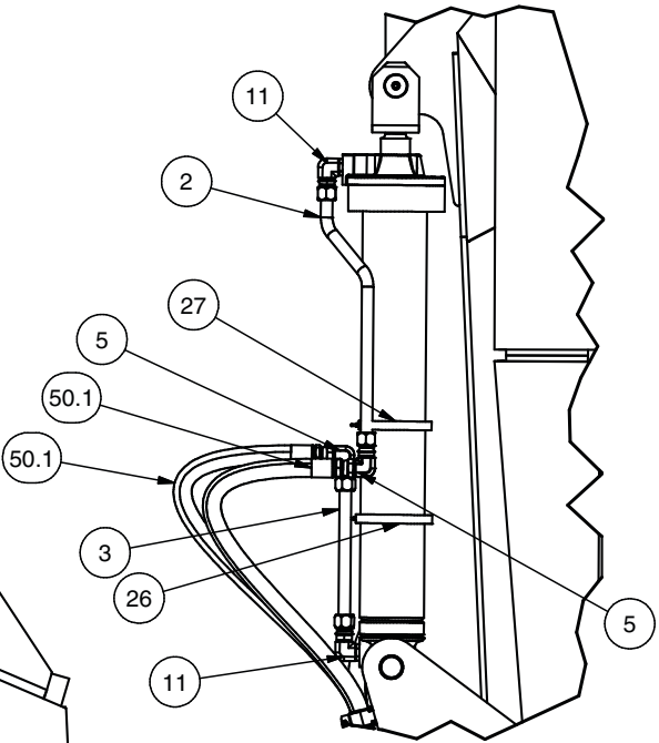
AUX HOLDDOWN DETAIL 1A 2 PLCS
