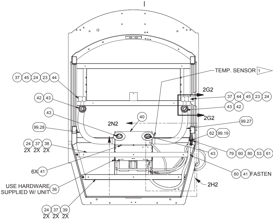
SECTION 2A1-2A1
