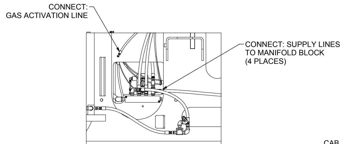
SECTION B-B SOME COMPONENTS NOT SHOWN FOR CLARITY
