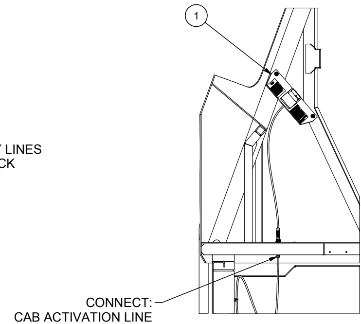
SECTION C-C SOME COMPONENTS NOT SHOWN FOR CLARITY
