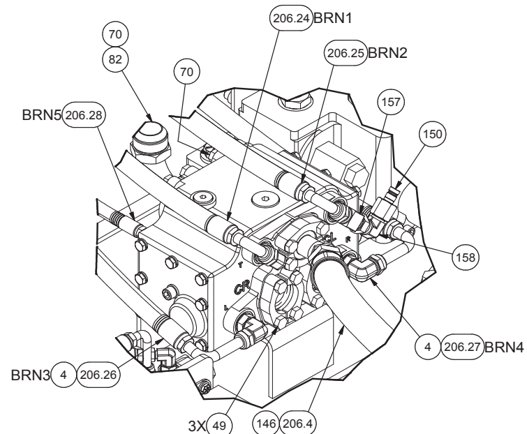
DETAIL 3J PARTS REMOVED FOR CLARITY
