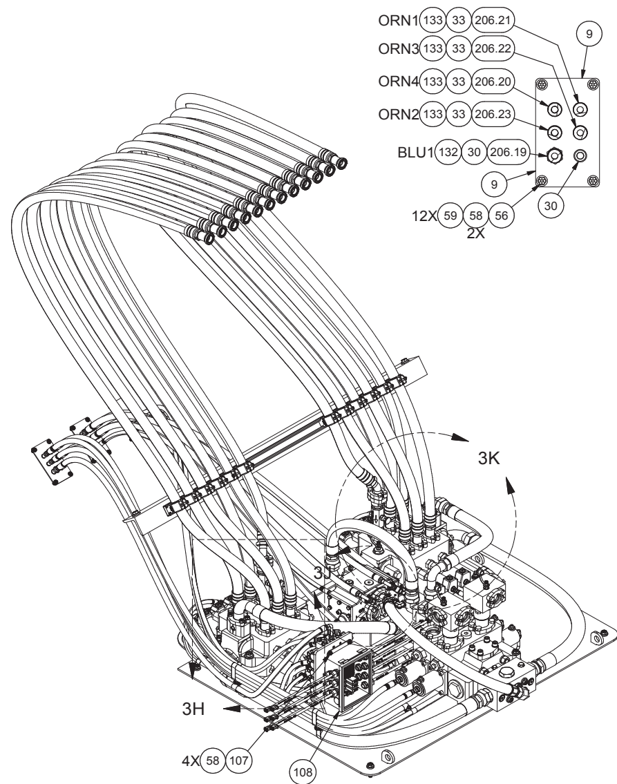
SECTION 3G-3G
