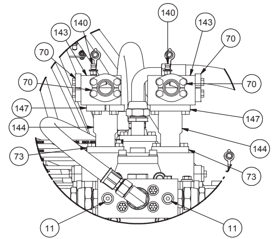
DETAIL 3C
