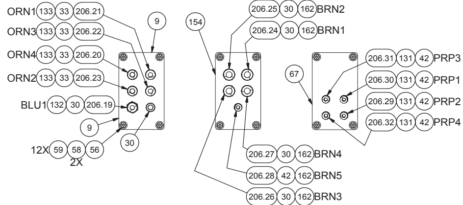
SECTION 3G-3G
