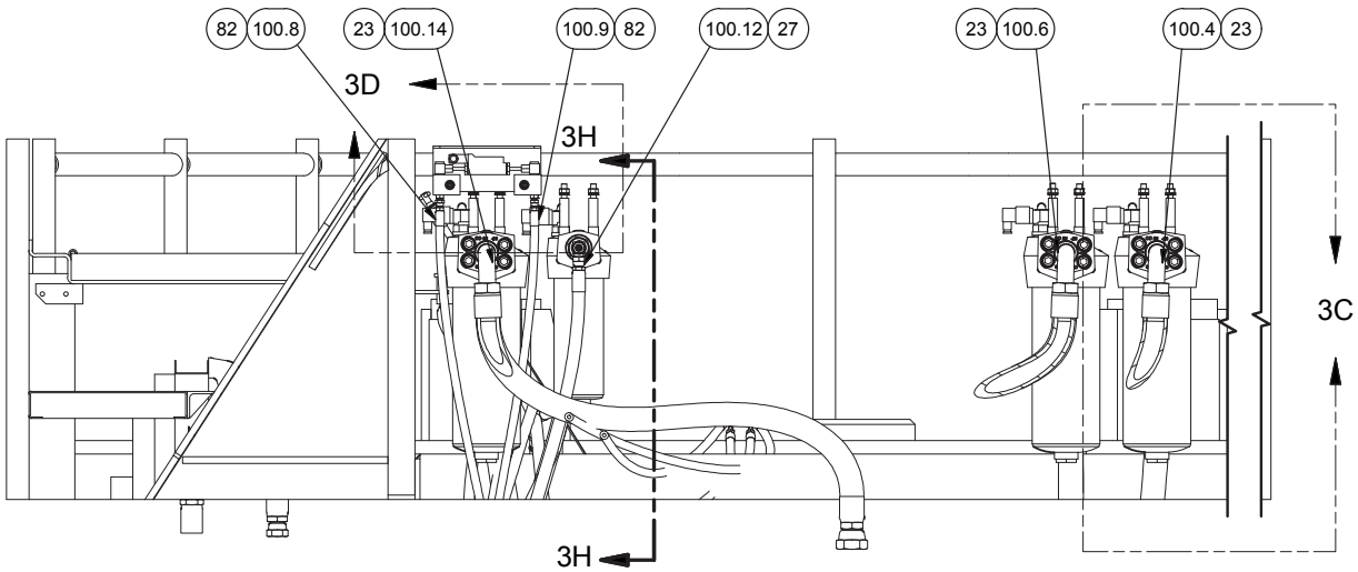
SECTION 3A-3A
