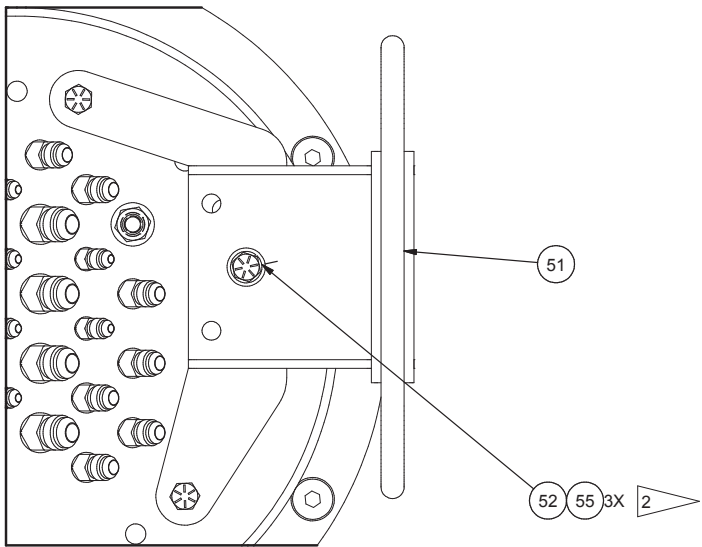
DETAIL B
