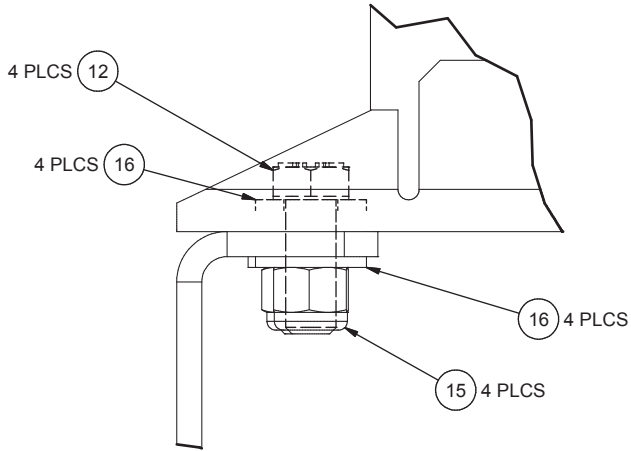
DETAIL A
