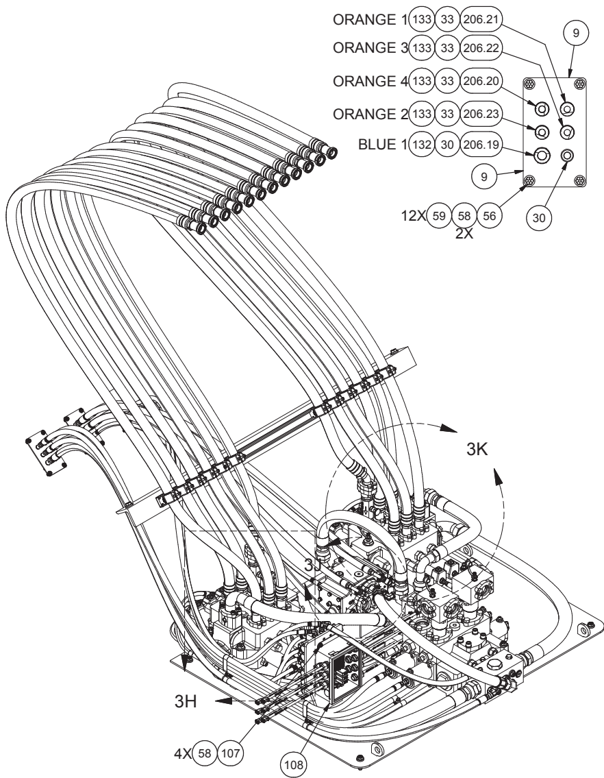
SECTION 3G-3G
