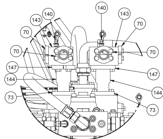
DETAIL 3C
