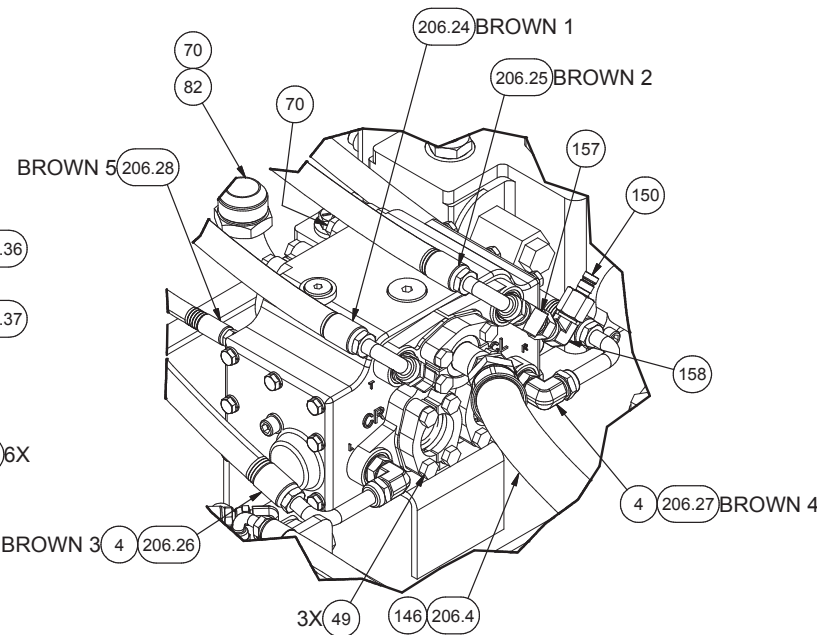
DETAIL 3J PARTS REMOVED FOR CLARITY
