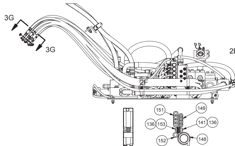
DETAIL 2F FLATTEN CLAMPS AS SHOWN
