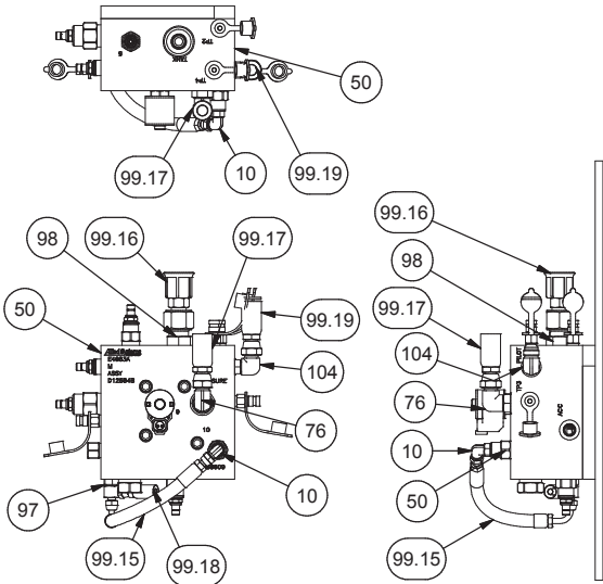
DETAIL 2H
