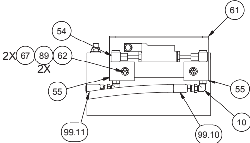
SECTION 2D-2D
