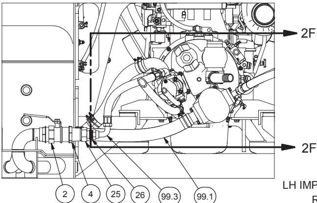
SECTION 2G-2G
