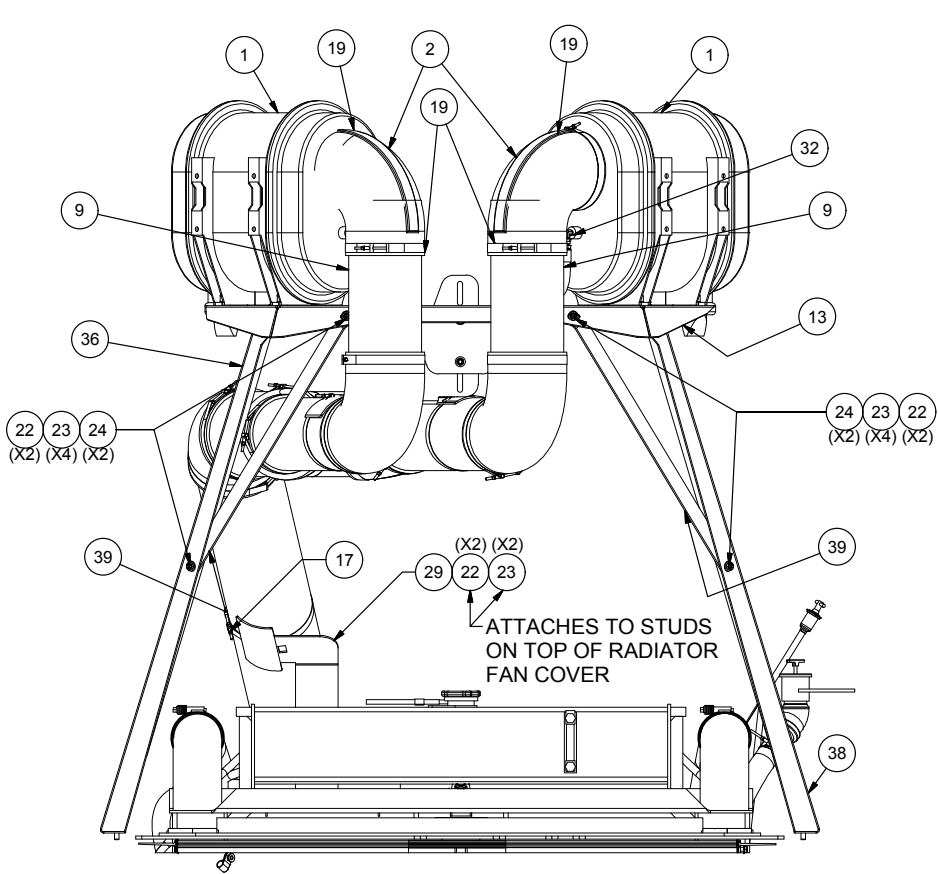
VIEW 2B-2B
