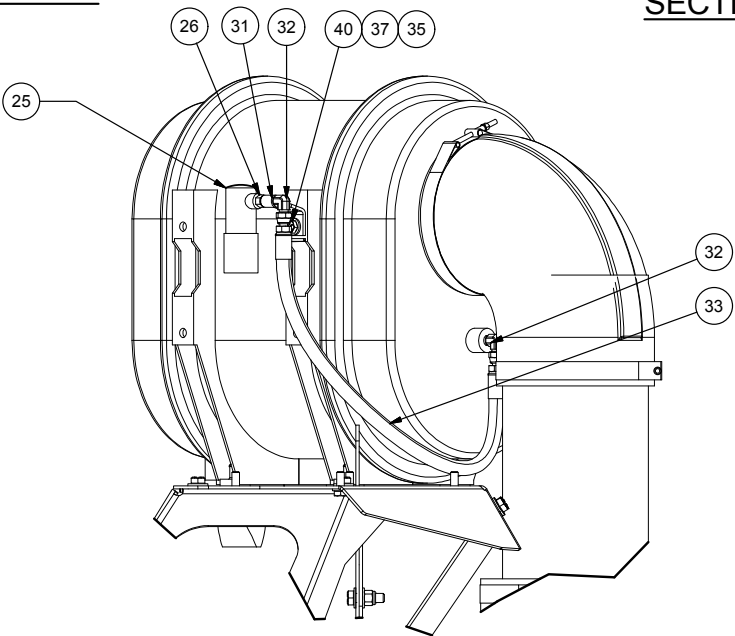
DETAIL 2E ITEM 1 (LEFT SIDE) REMOVED FROM VIEW FOR CLARITY OF AIR INDICATOR (ITEM 25) HOSE ROUTING
