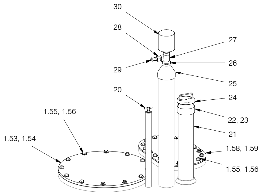
DETAIL B
