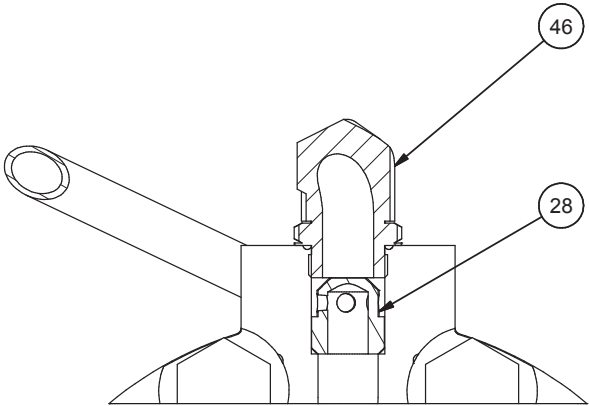
SECTION B-B BOTH TILT CYL
