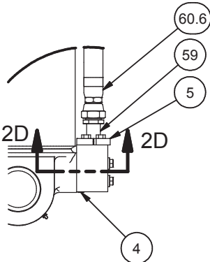
DETAIL 2C
