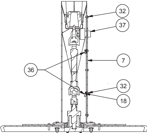
SECTION A1-A1
