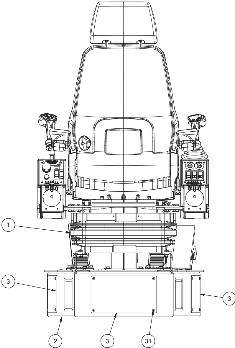
SECTION A1-A1
