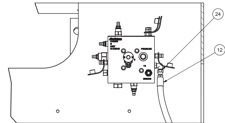
DETAIL 3G PICTORIAL REPRESENTATION OF ACC/PILOT MANIFOLD: MAY CHANGE
