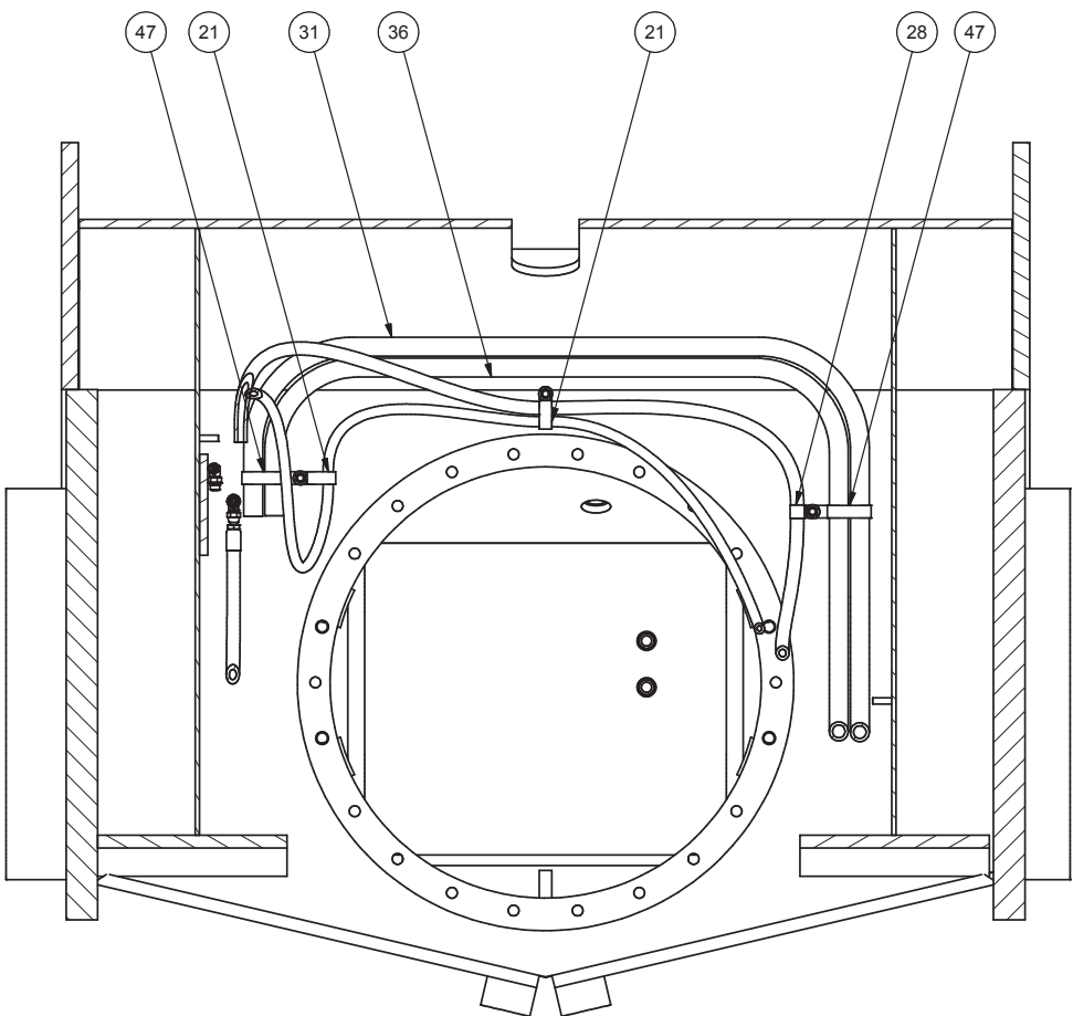
SECTION 4H-4H
