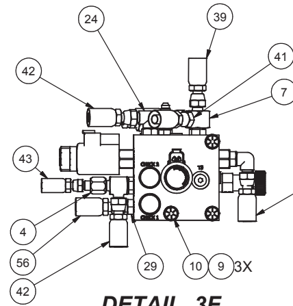
DETAIL 3F
