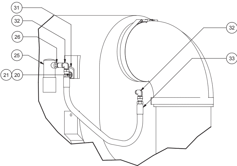
DETAIL E ITEM 1 (LEFT SIDE) REMOVED FROM VIEW FOR CLARITY OF AIR INDICATOR (ITEM 25) HOSE ROUTING
