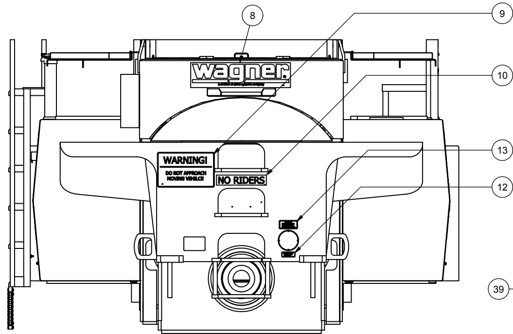
VIEW 2C-2C
