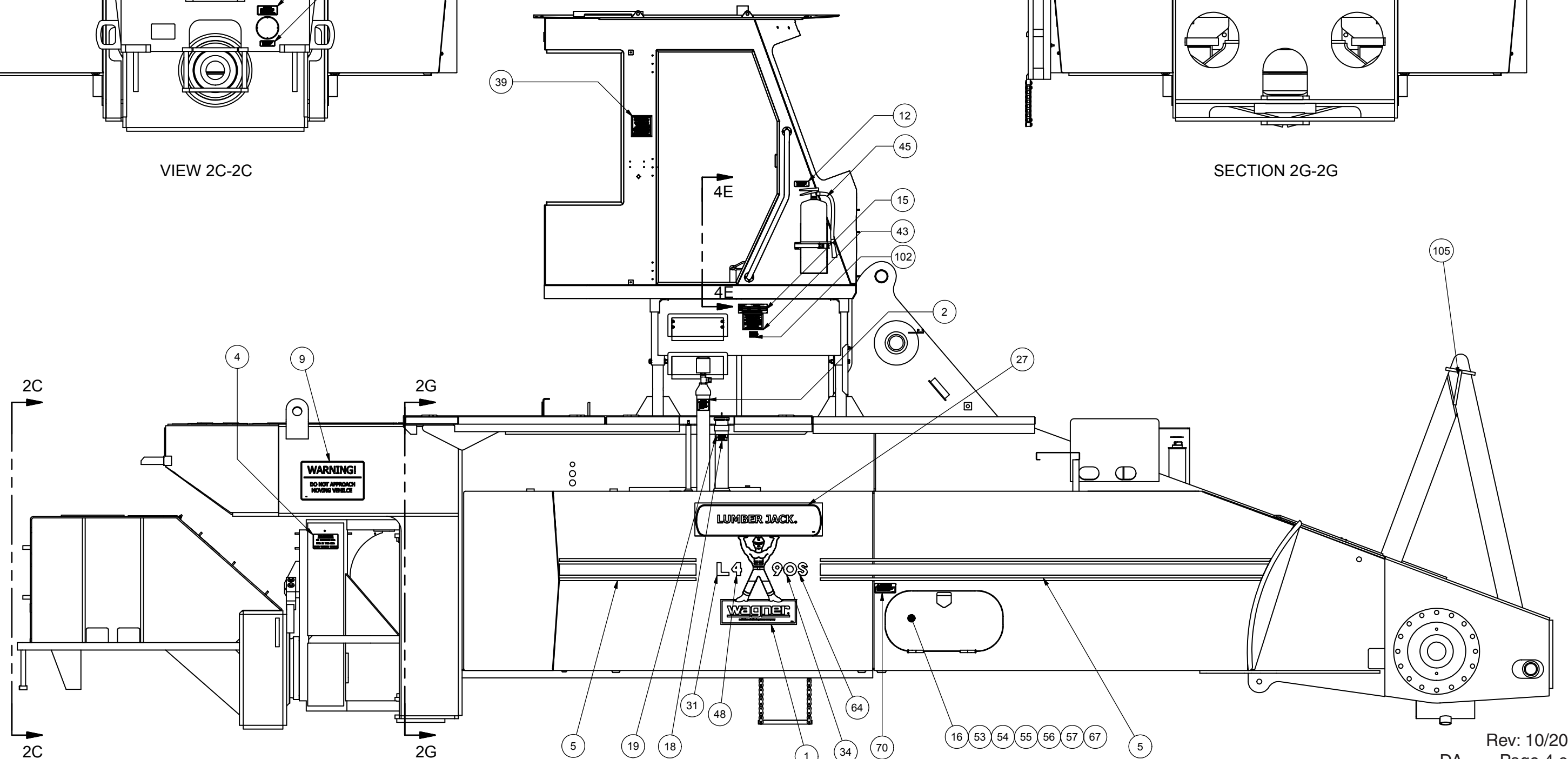
VIEW 2A-2A
