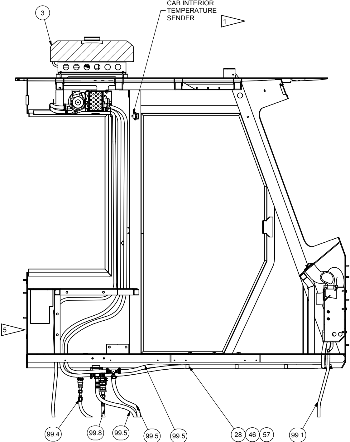
SECTION 3J-3J
